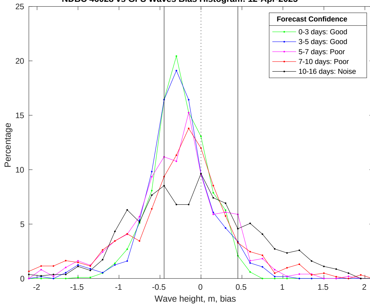
NDBC 46028 vs GFS Waves Bias Histogram: 12-Apr-2025
