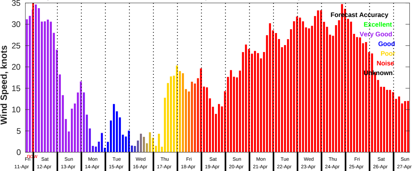
GFS Wind Speed Forecast for NDBC 46028 from 11-Apr-2025 16:00:00 to 27-Apr-2025 16:00:00
