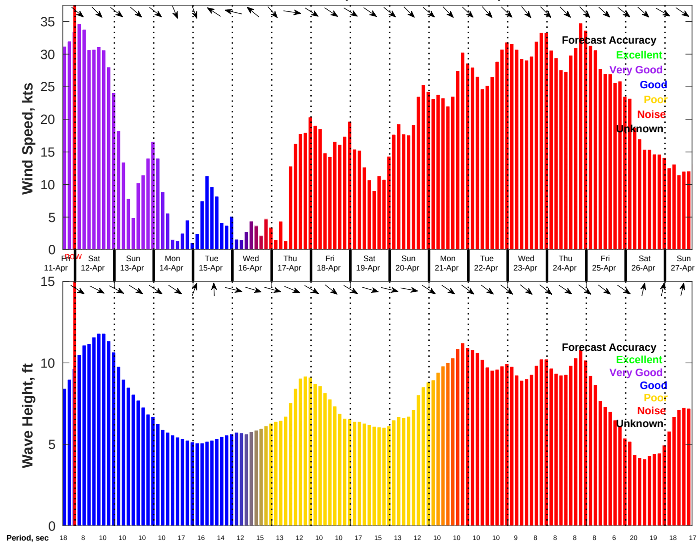
Wind & Wave Forecast for NDBC 46028 from 11-Apr-2025 16:00:00 to 27-Apr-2025 16:00:00
