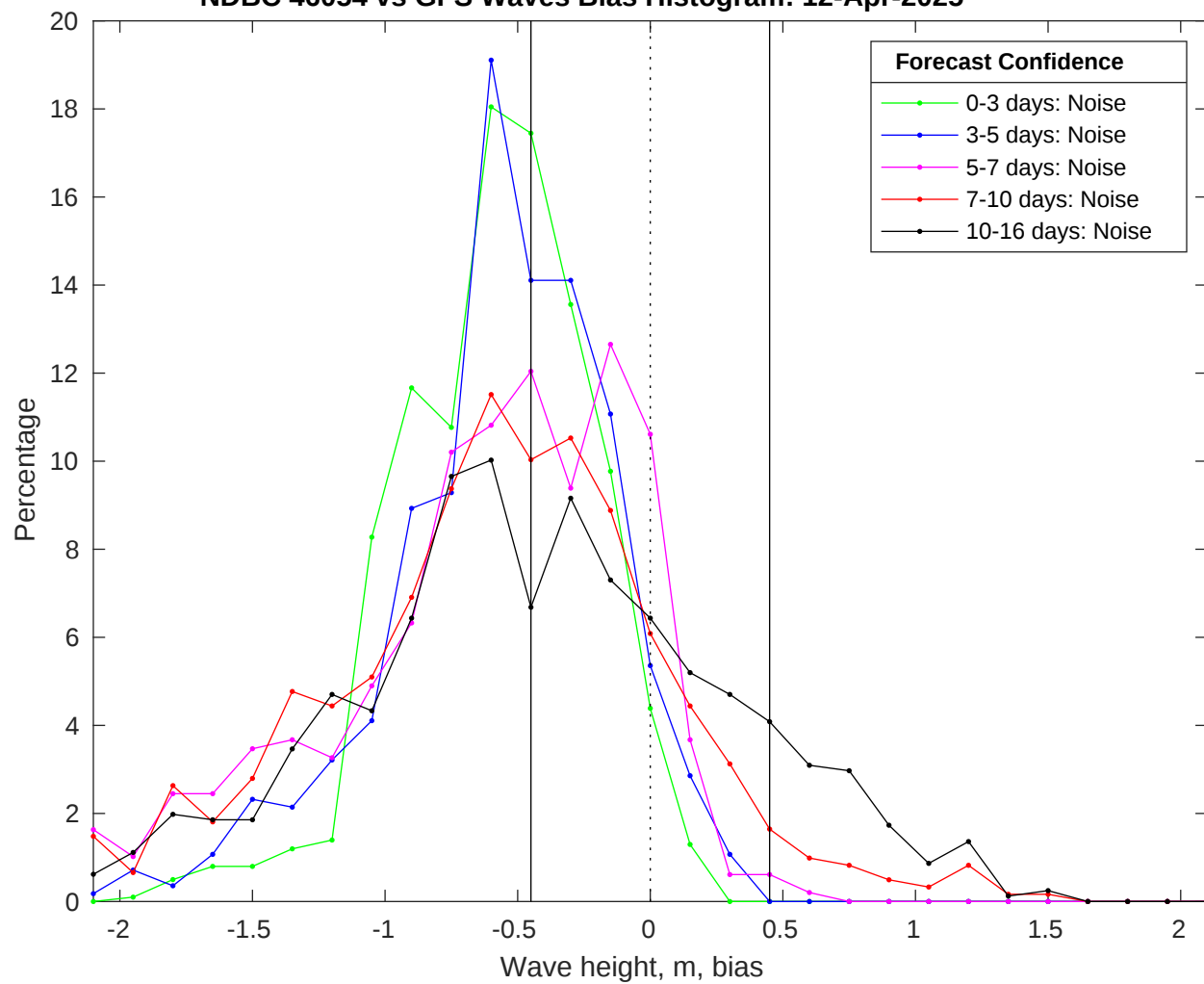
NDBC 46054 vs GFS Waves Bias Histogram: 12-Apr-2025
