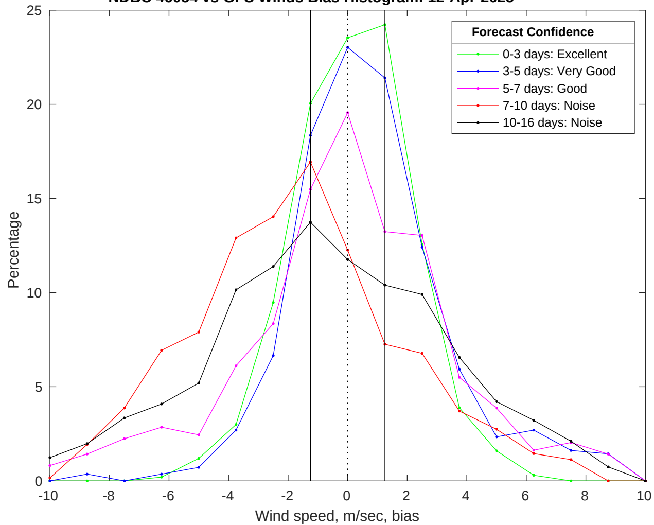
NDBC 46054 vs GFS Winds Bias Histogram: 12-Apr-2025
