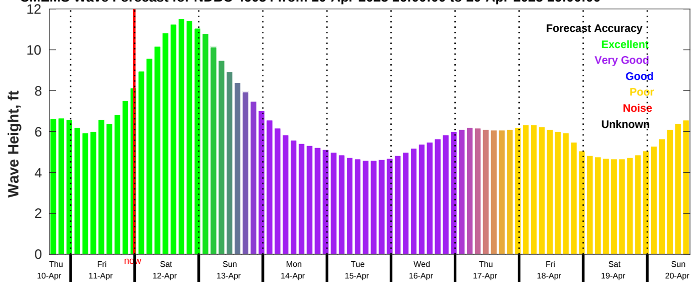
CMEMS Wave Forecast for NDBC 46054 from 10-Apr-2025 16:00:00 to 20-Apr-2025 16:00:00
