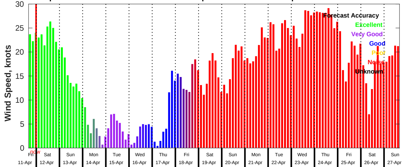
GFS Wind Speed Forecast for NDBC 46054 from 11-Apr-2025 16:00:00 to 27-Apr-2025 16:00:00
