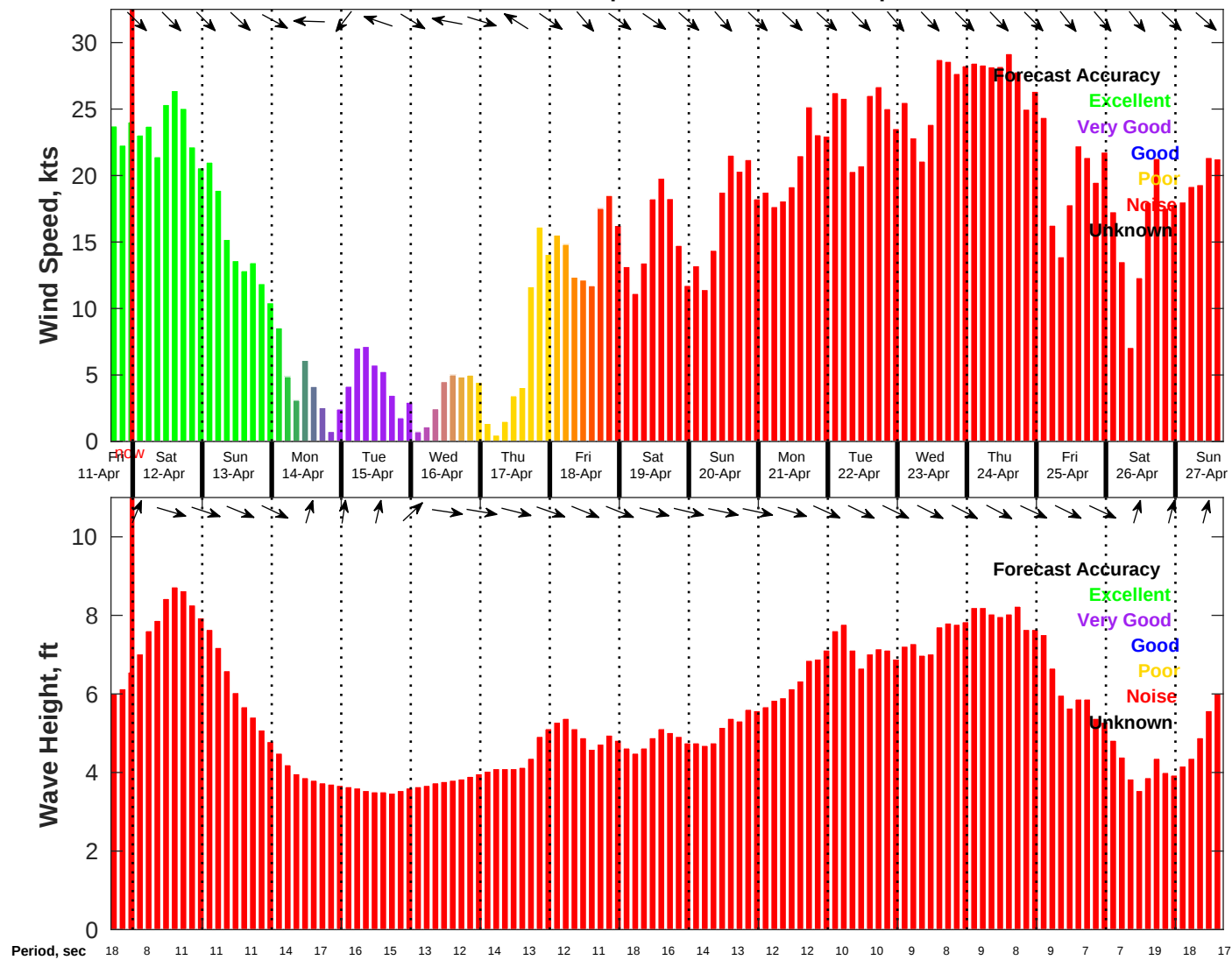
Wind & Wave Forecast for NDBC 46054 from 11-Apr-2025 16:00:00 to 27-Apr-2025 16:00:00
