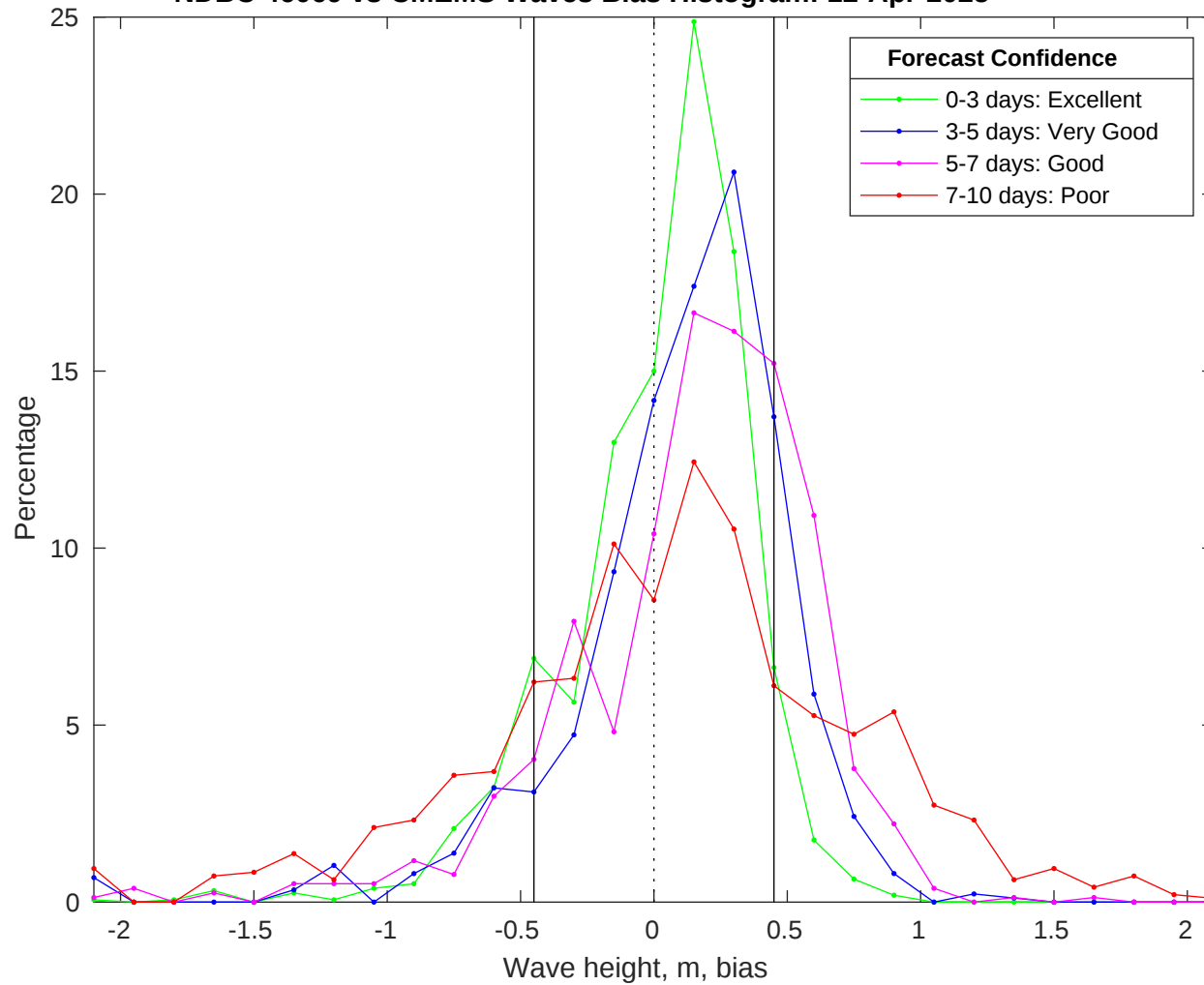
NDBC 46069 vs CMEMS Waves Bias Histogram: 12-Apr-2025
