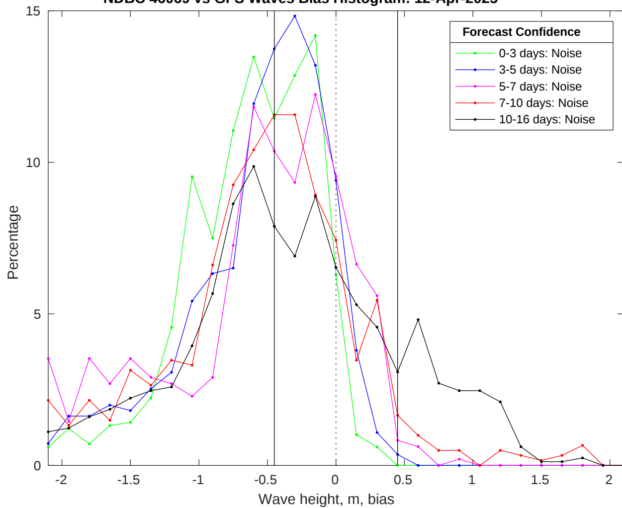
NDBC 46069 vs GFS Waves Bias Histogram: 12-Apr-2025
