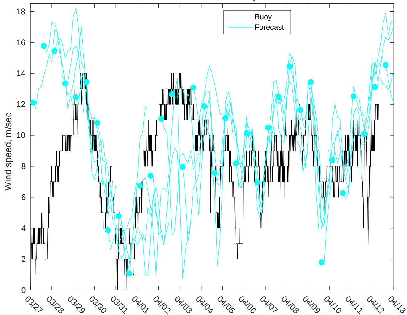
NDBC 46069 vs GFS Winds: 5 to 7 day forecast
