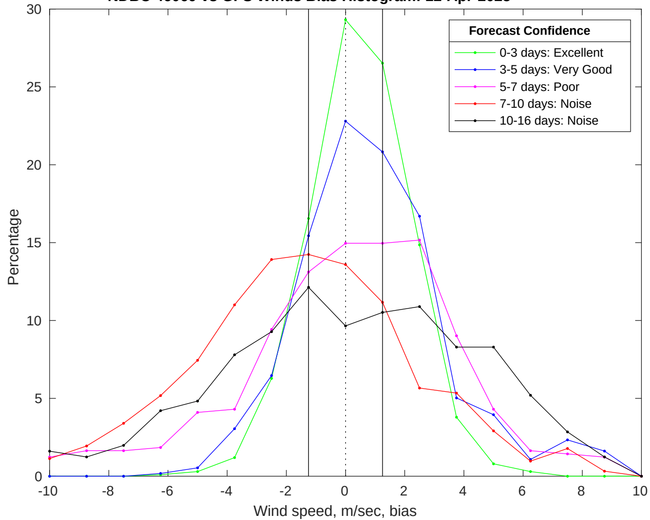
NDBC 46069 vs GFS Winds Bias Histogram: 12-Apr-2025
