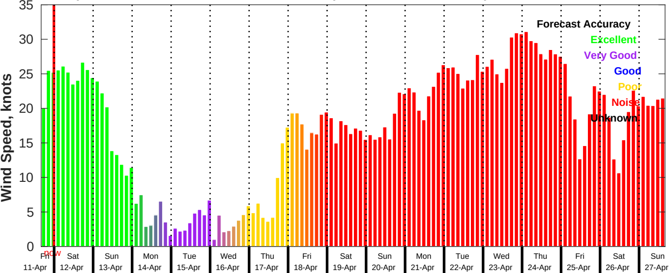
GFS Wind Speed Forecast for NDBC 46069 from 11-Apr-2025 16:00:00 to 27-Apr-2025 16:00:00
