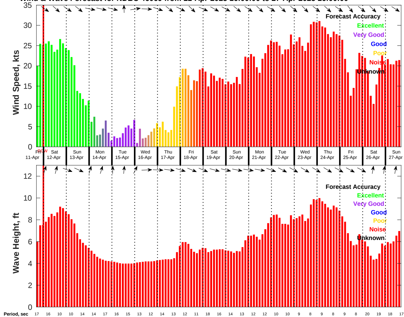
Wind & Wave Forecast for NDBC 46069 from 11-Apr-2025 16:00:00 to 27-Apr-2025 16:00:00
