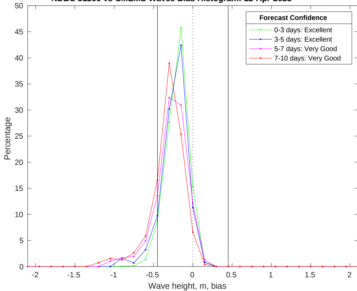
NDBC 51209 vs CMEMS Waves Bias Histogram: 12-Apr-2025
