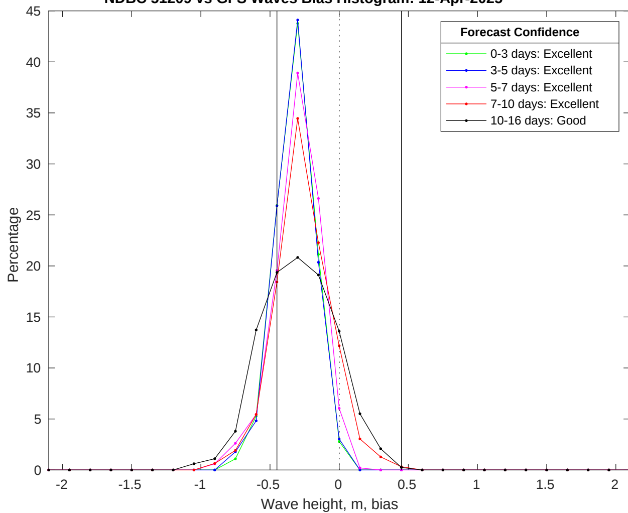
NDBC 51209 vs GFS Waves Bias Histogram: 12-Apr-2025
