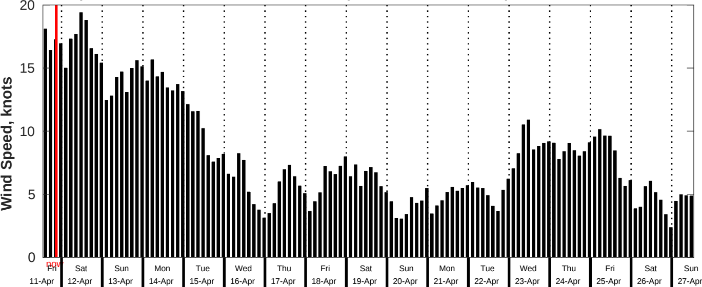
GFS Wind Speed Forecast for NDBC 51209 from 11-Apr-2025 13:00:00 to 27-Apr-2025 13:00:00
