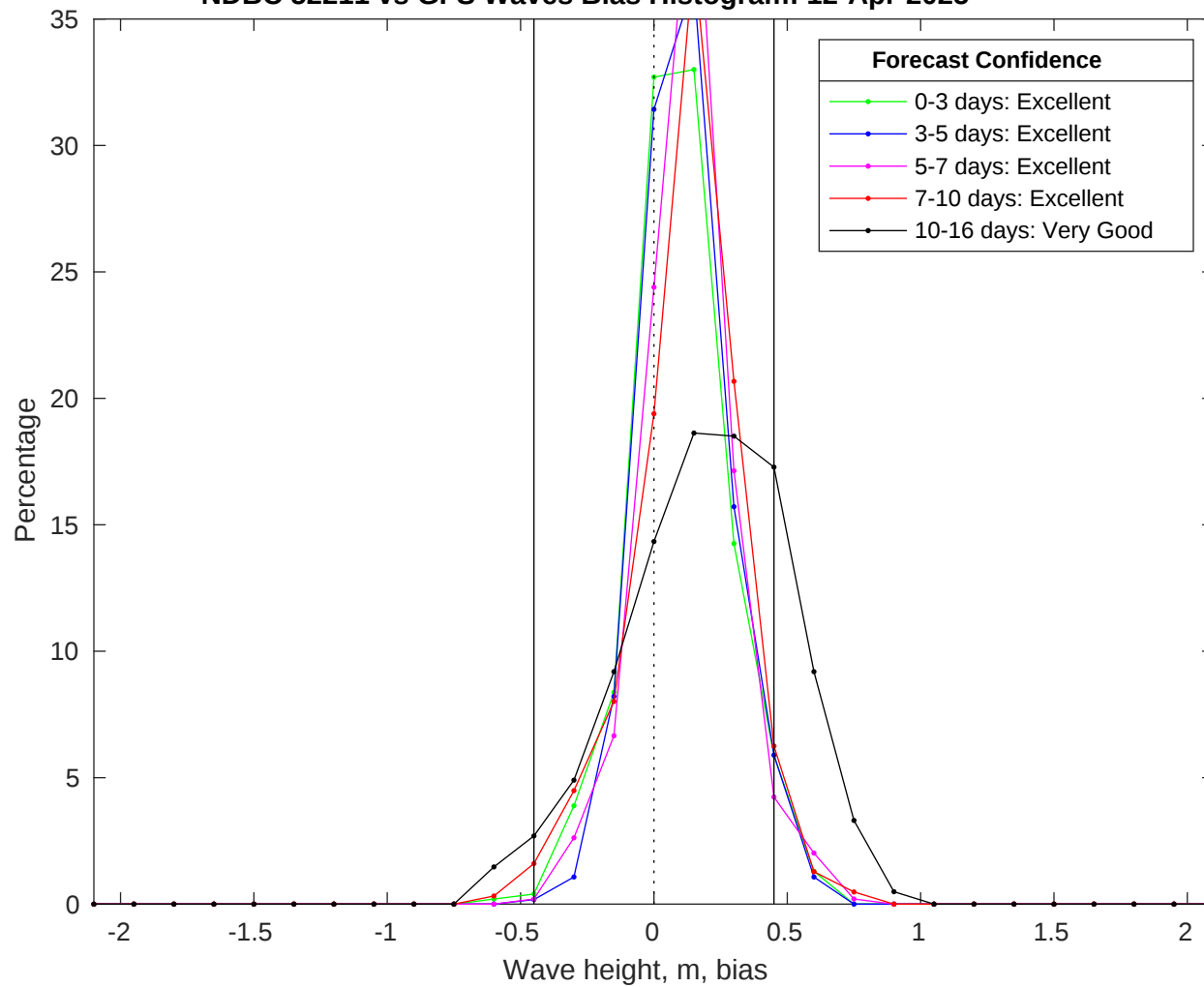
NDBC 52211 vs GFS Waves Bias Histogram: 12-Apr-2025
