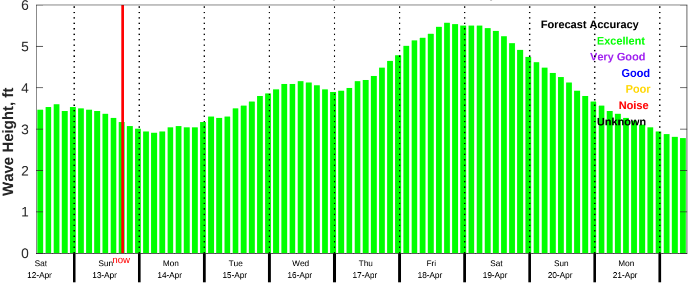
CMEMS Wave Forecast for NDBC 52211 from 11-Apr-2025 10:00:00 to 21-Apr-2025 10:00:00
