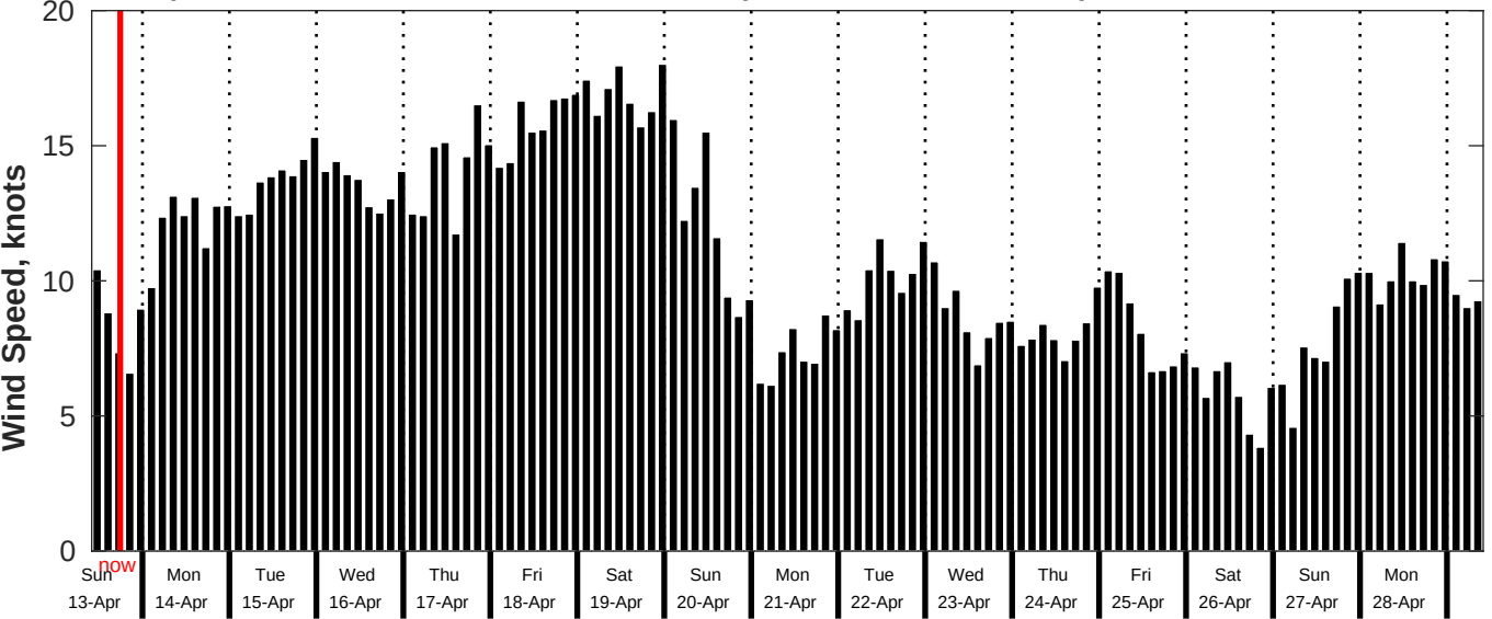
GFS Wind Speed Forecast for NDBC 52211 from 12-Apr-2025 10:00:00 to 28-Apr-2025 10:00:00
