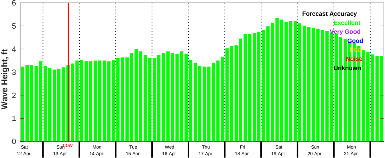
CMEMS Wave Forecast for NDBC 52212 from 11-Apr-2025 09:00:00 to 21-Apr-2025 09:00:00
