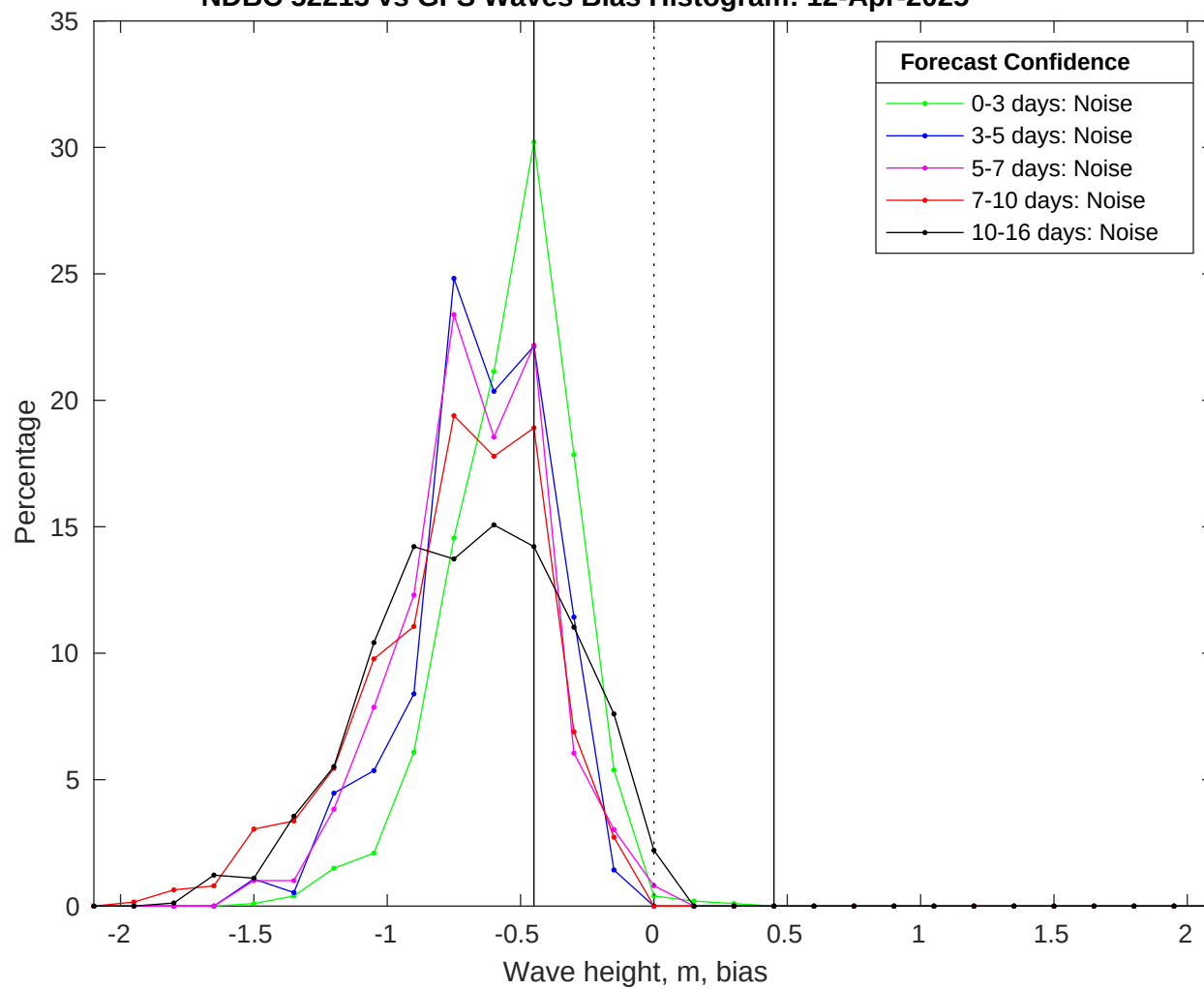
NDBC 52213 vs GFS Waves Bias Histogram: 12-Apr-2025
