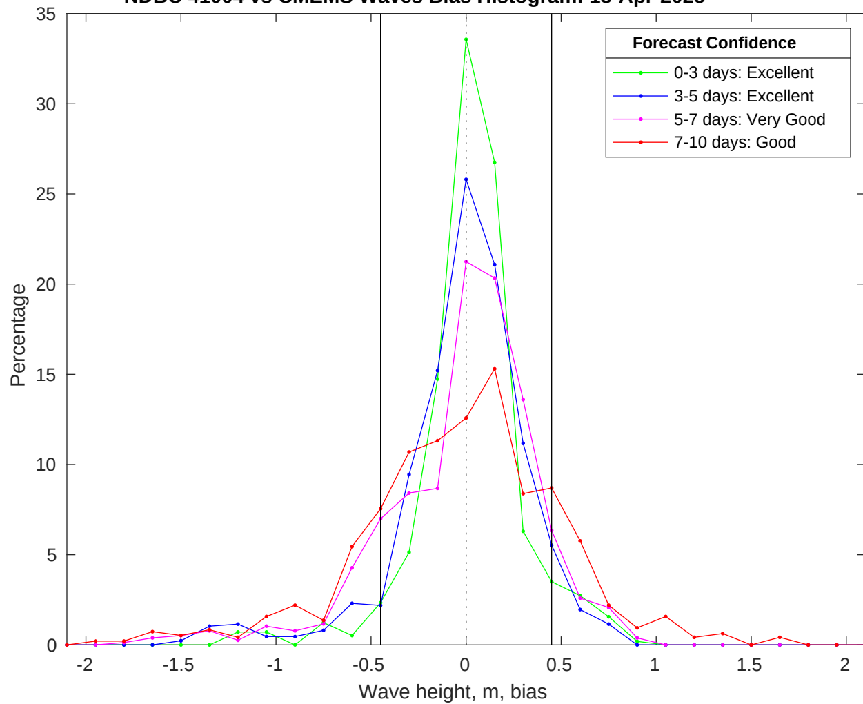
NDBC 41004 vs CMEMS Waves Bias Histogram: 13-Apr-2025
