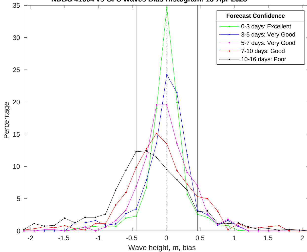
NDBC 41004 vs GFS Waves Bias Histogram: 13-Apr-2025
