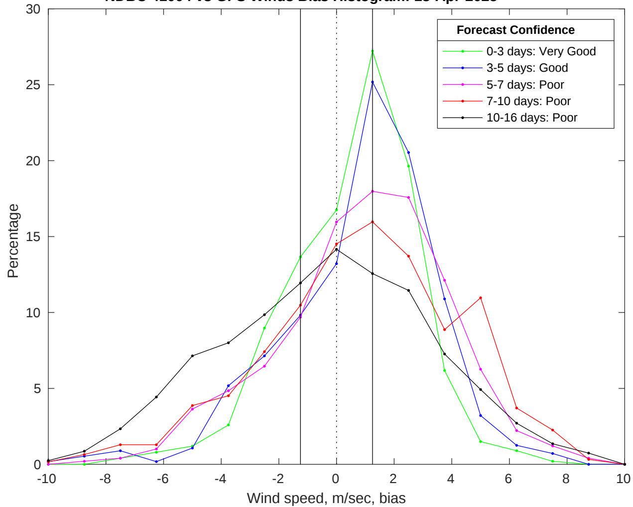
NDBC 41004 vs GFS Winds Bias Histogram: 13-Apr-2025
