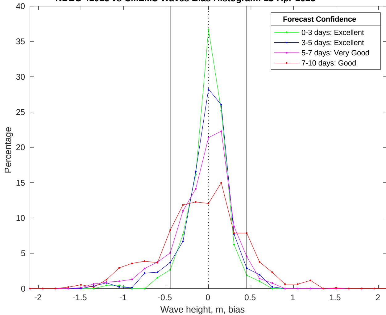
NDBC 41013 vs CMEMS Waves Bias Histogram: 13-Apr-2025
