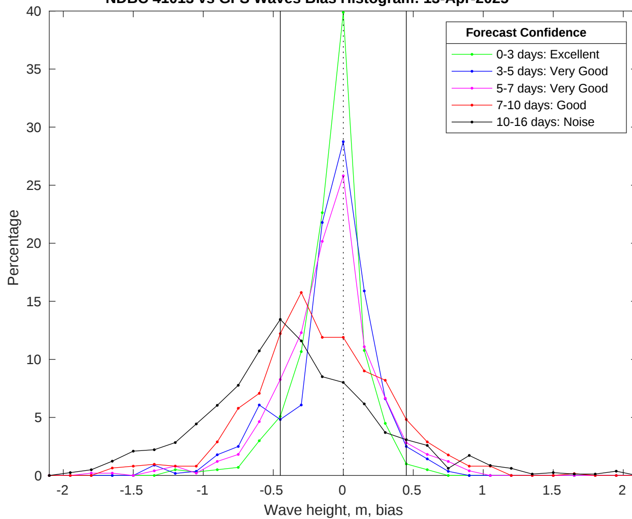
NDBC 41013 vs GFS Waves Bias Histogram: 13-Apr-2025
