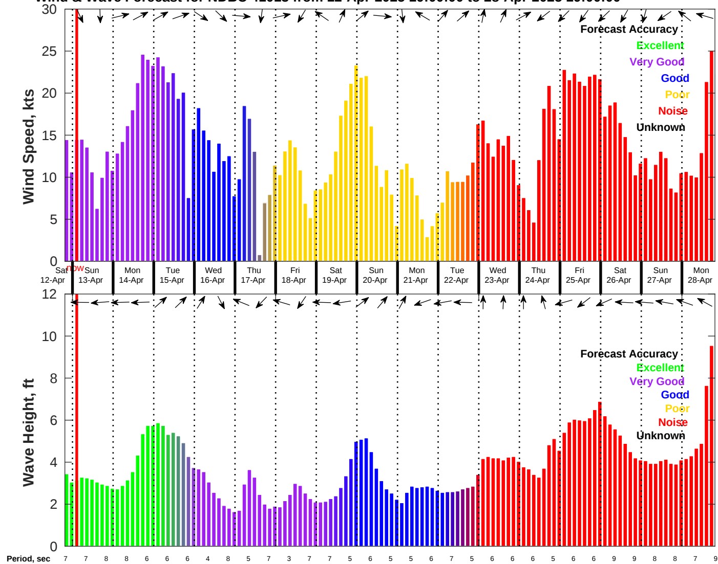
Wind & Wave Forecast for NDBC 41013 from 12-Apr-2025 19:00:00 to 28-Apr-2025 19:00:00
