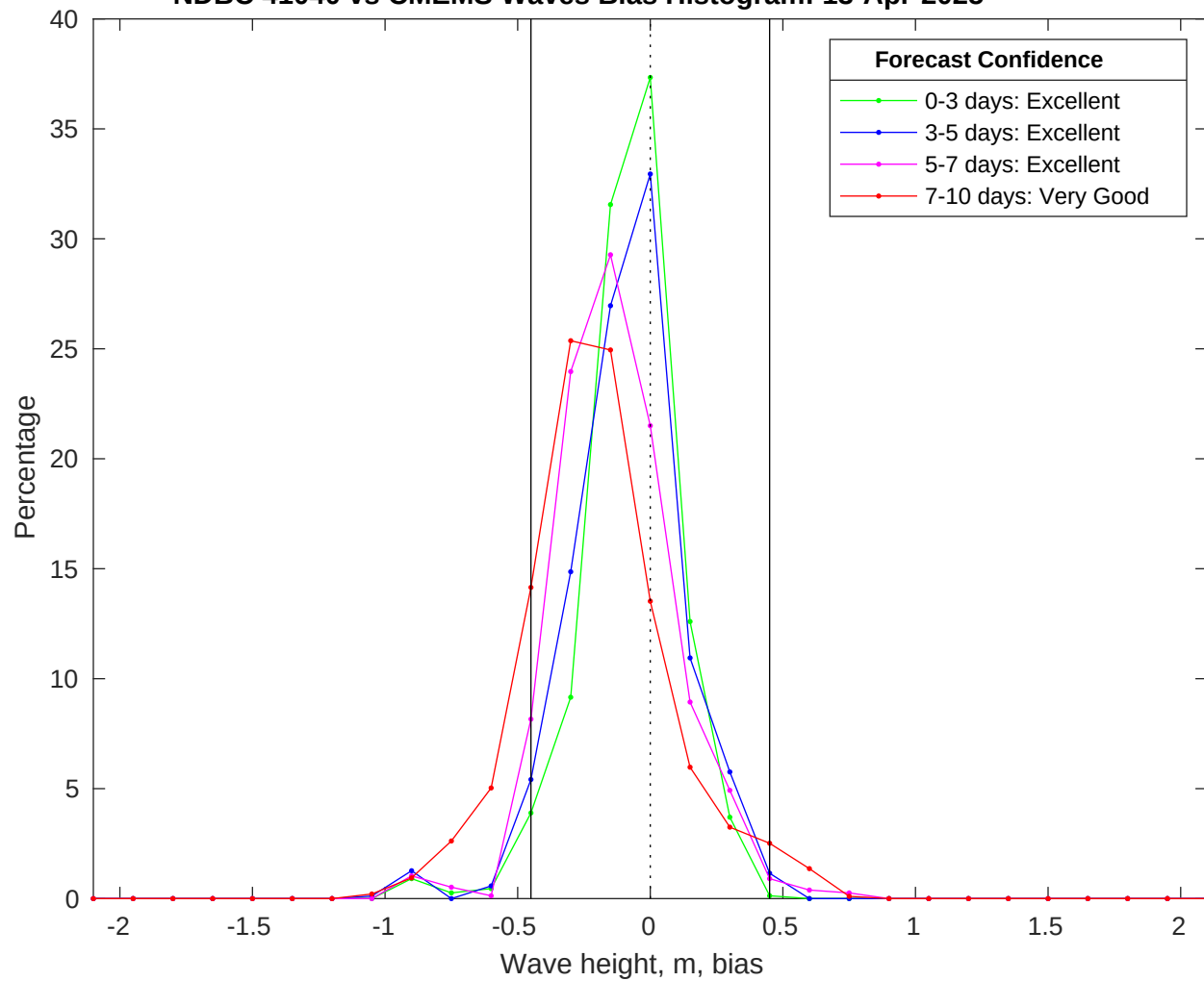
NDBC 41040 vs CMEMS Waves Bias Histogram: 13-Apr-2025
