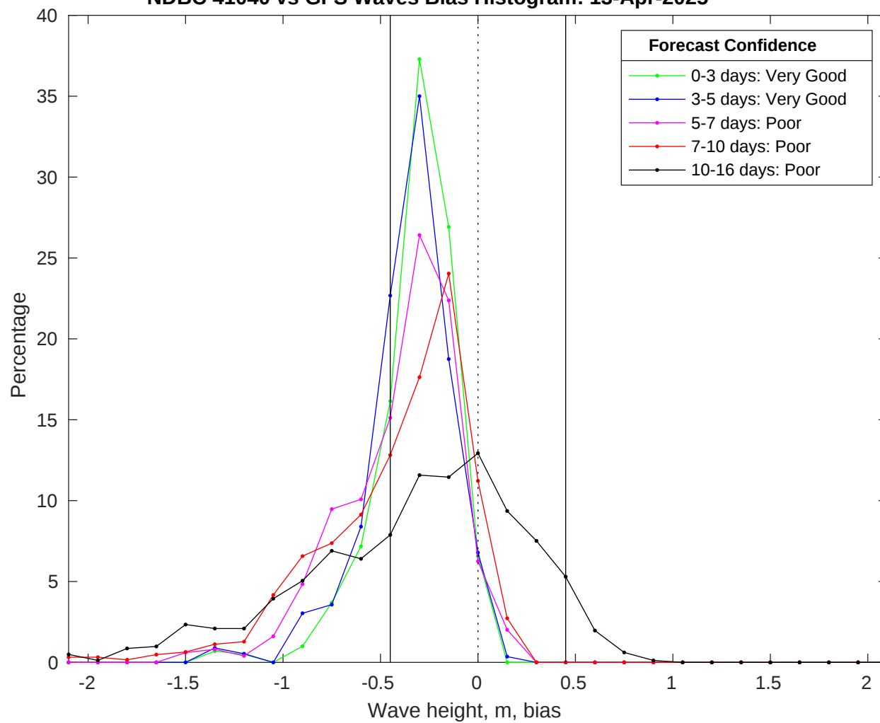
NDBC 41040 vs GFS Waves Bias Histogram: 13-Apr-2025
