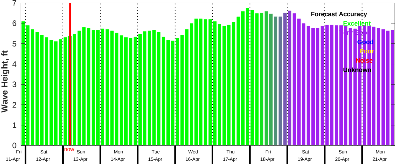
CMEMS Wave Forecast for NDBC 41040 from 11-Apr-2025 21:00:00 to 21-Apr-2025 21:00:00
