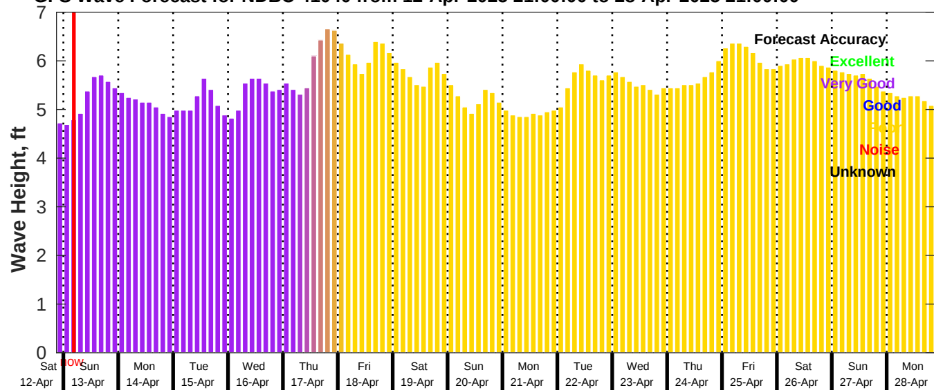
GFS Wave Forecast for NDBC 41040 from 12-Apr-2025 21:00:00 to 28-Apr-2025 21:00:00
