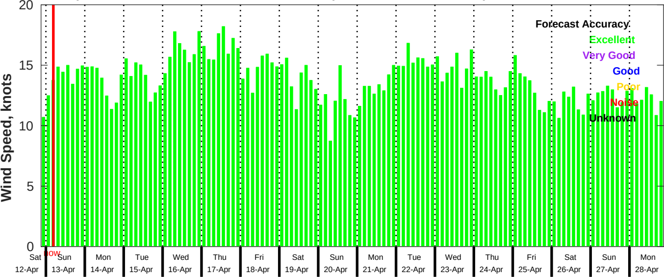
GFS Wind Speed Forecast for NDBC 41040 from 12-Apr-2025 21:00:00 to 28-Apr-2025 21:00:00
