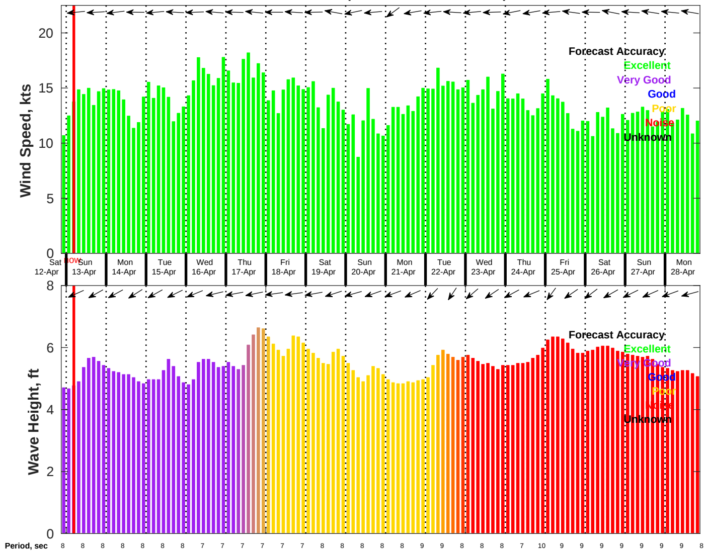
Wind & Wave Forecast for NDBC 41040 from 12-Apr-2025 21:00:00 to 28-Apr-2025 21:00:00
