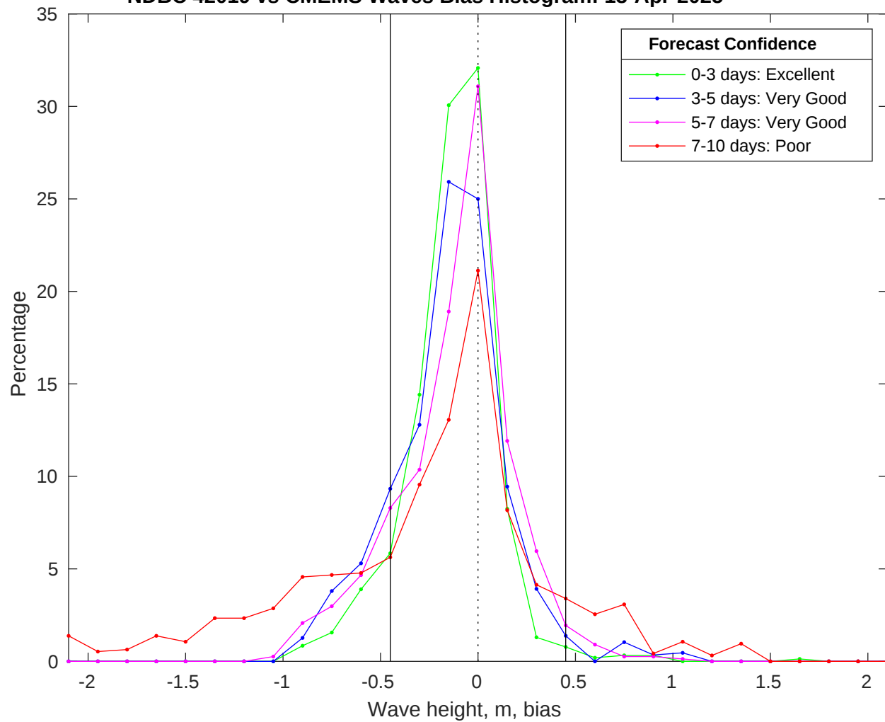
NDBC 42019 vs CMEMS Waves Bias Histogram: 13-Apr-2025
