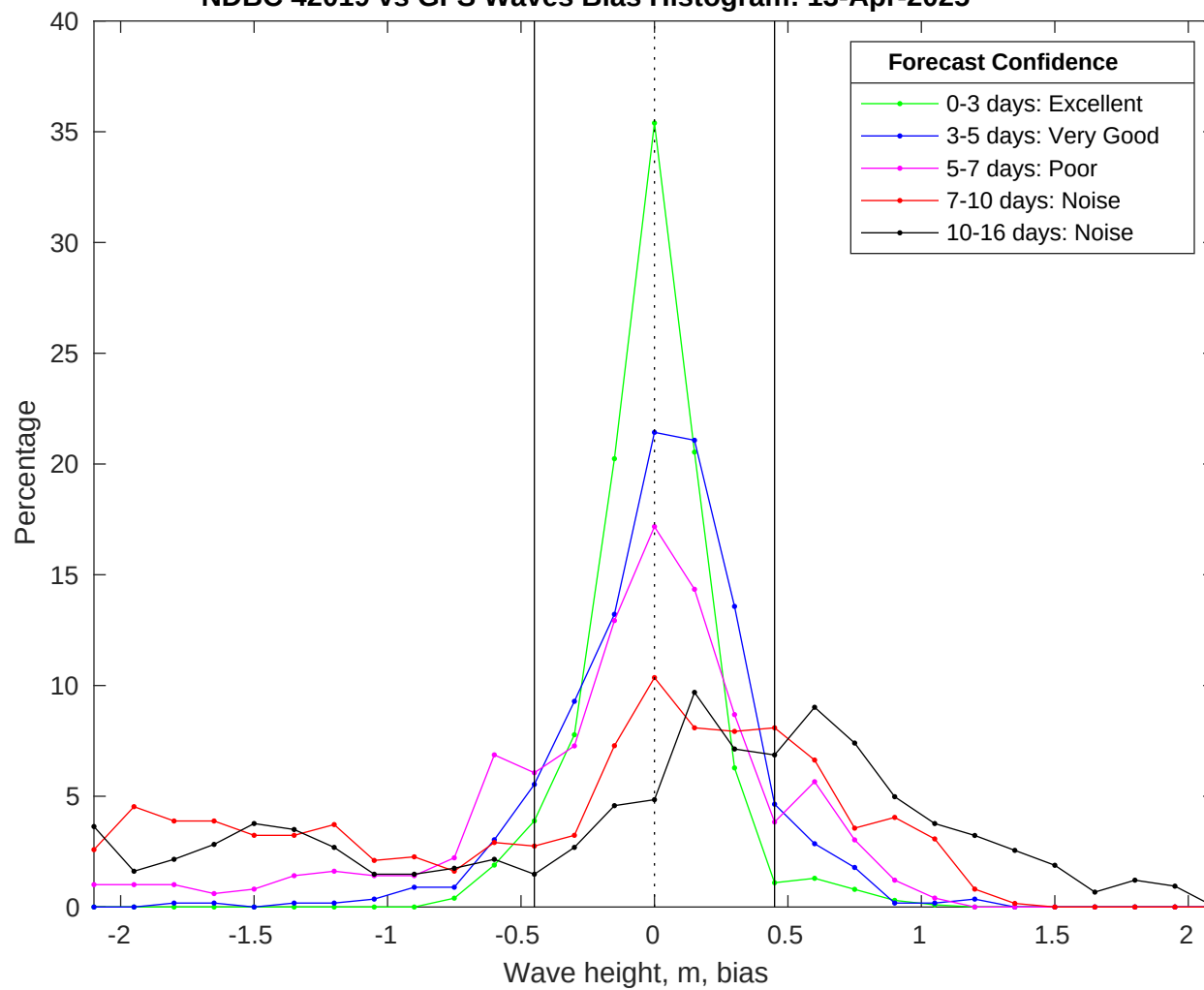
NDBC 42019 vs GFS Waves Bias Histogram: 13-Apr-2025
