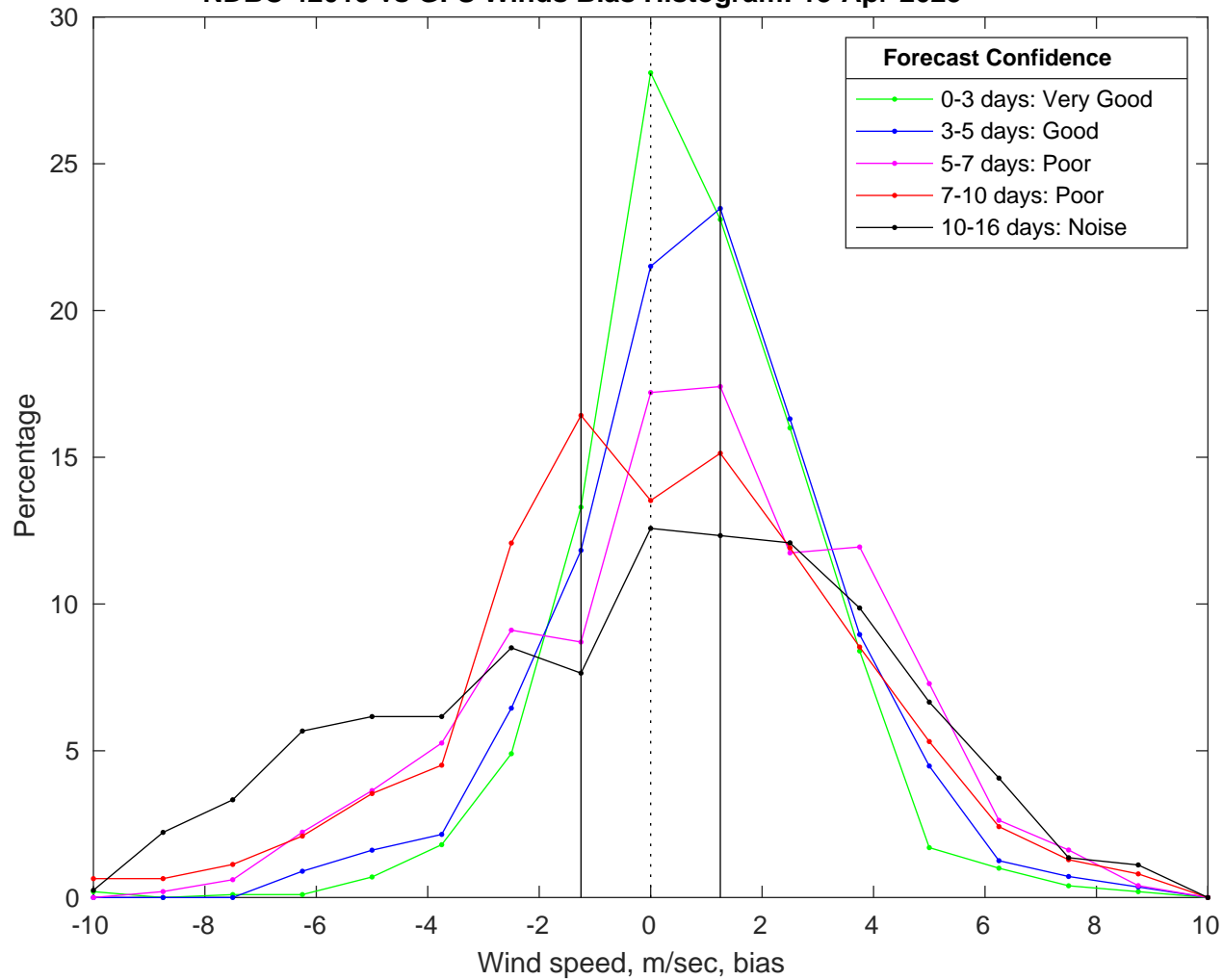
NDBC 42019 vs GFS Winds Bias Histogram: 13-Apr-2025
