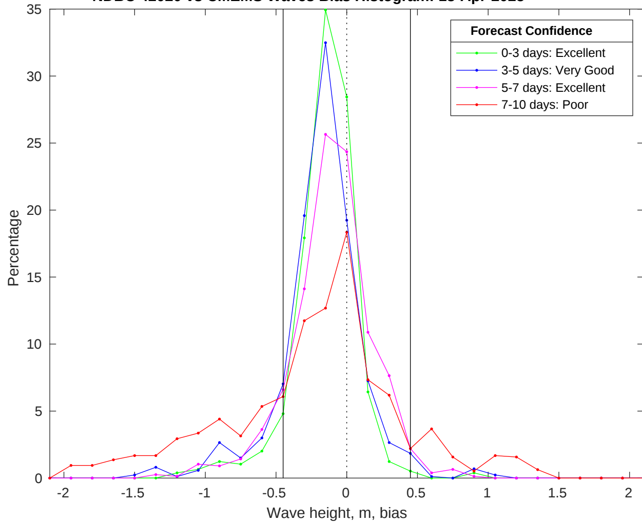
NDBC 42020 vs CMEMS Waves Bias Histogram: 13-Apr-2025
