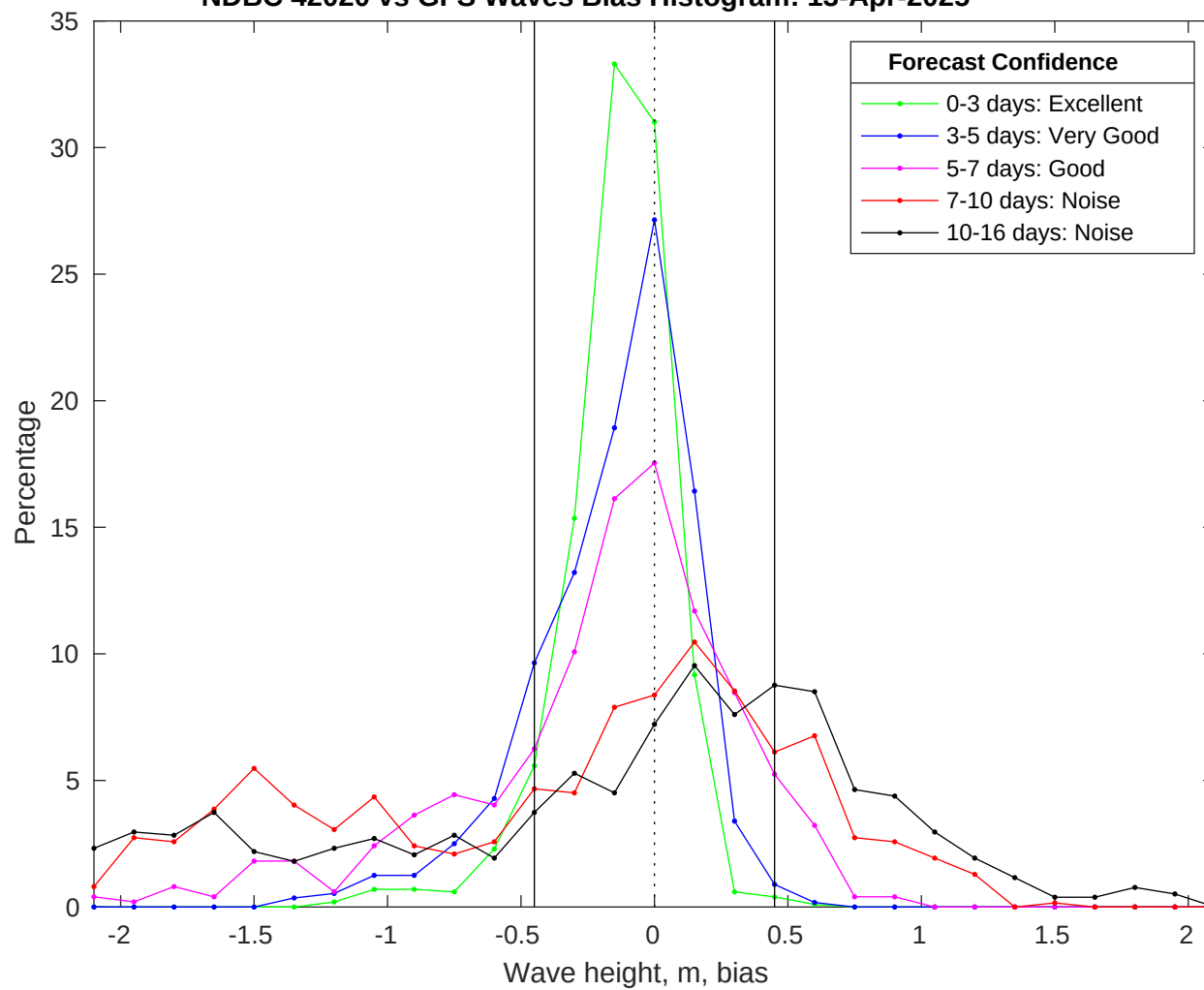
NDBC 42020 vs GFS Waves Bias Histogram: 13-Apr-2025
