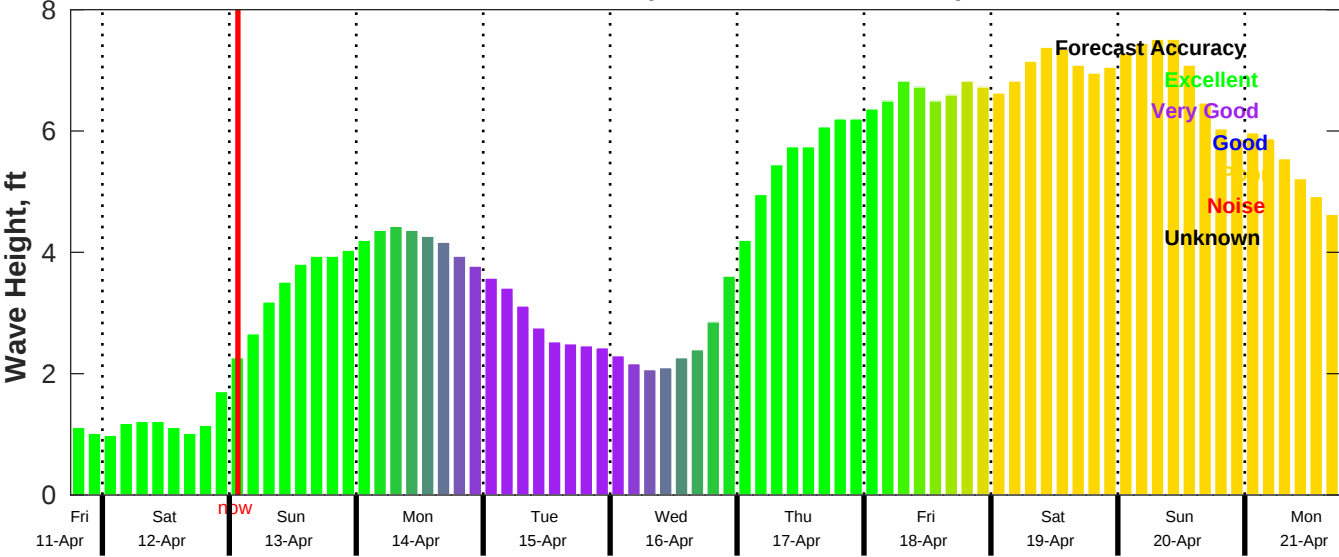
CMEMS Wave Forecast for NDBC 42020 from 11-Apr-2025 18:00:00 to 21-Apr-2025 18:00:00
