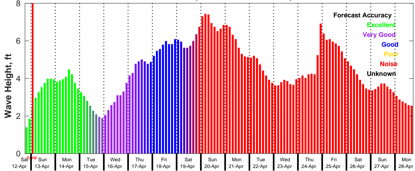
GFS Wave Forecast for NDBC 42020 from 12-Apr-2025 18:00:00 to 28-Apr-2025 18:00:00
