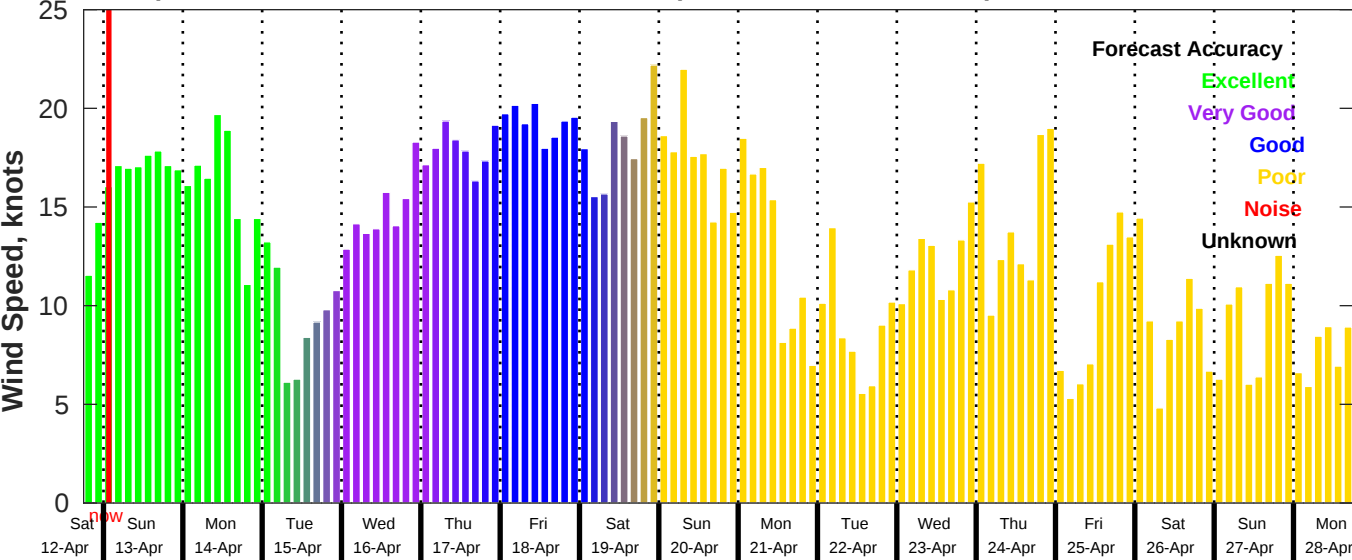
GFS Wind Speed Forecast for NDBC 42020 from 12-Apr-2025 18:00:00 to 28-Apr-2025 18:00:00
