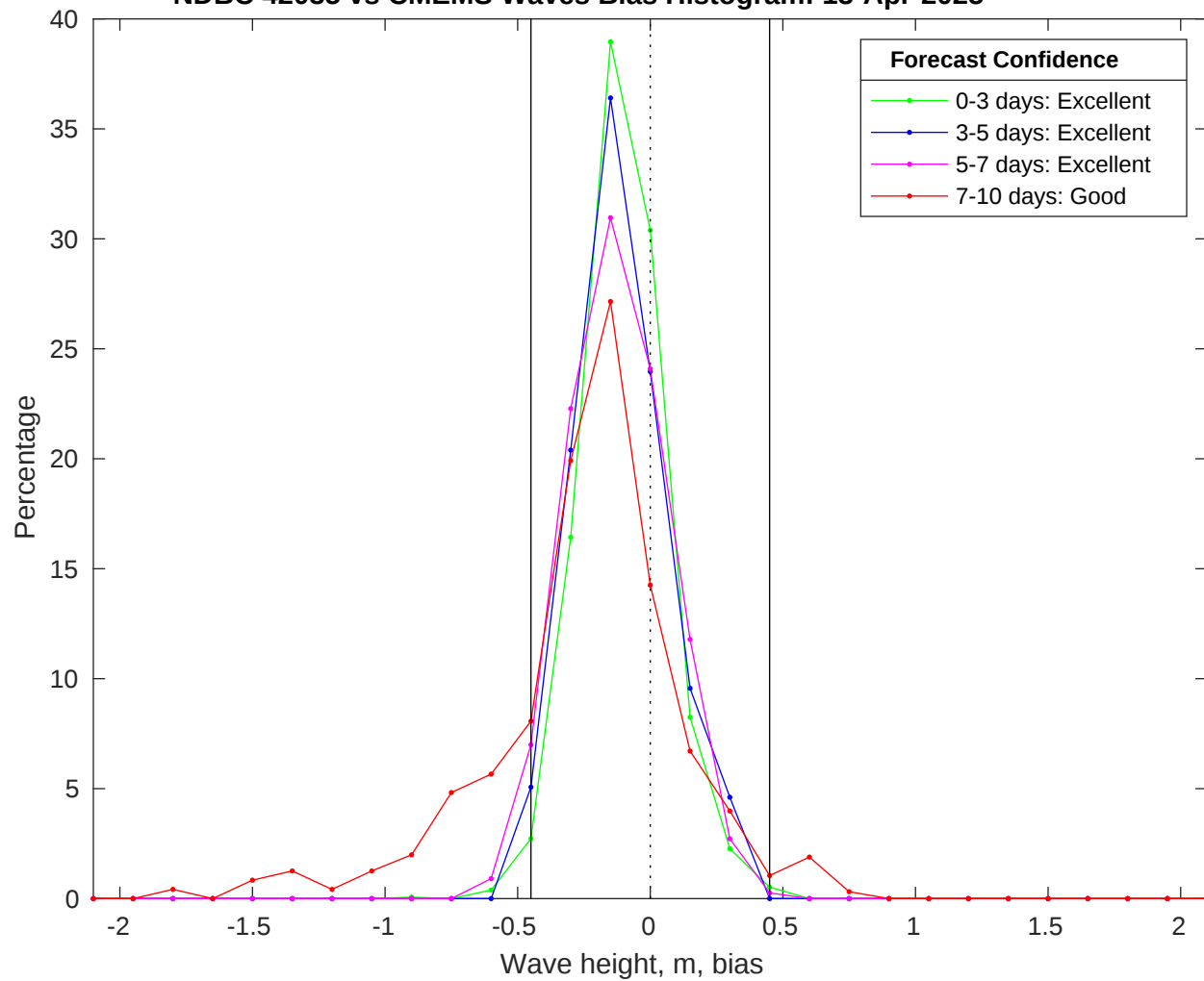
NDBC 42035 vs CMEMS Waves Bias Histogram: 13-Apr-2025
