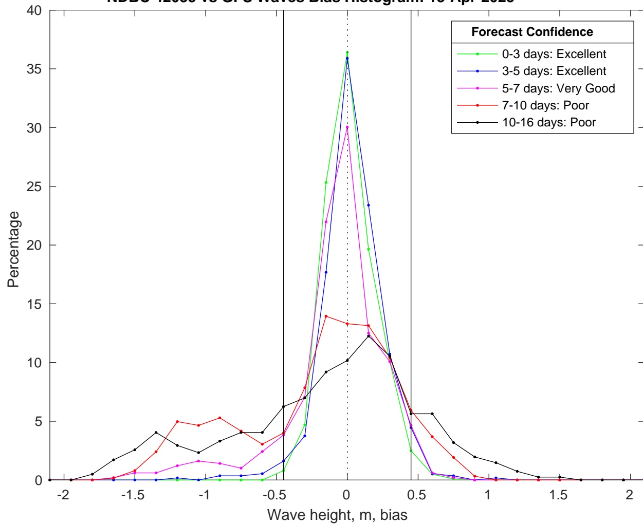
NDBC 42035 vs GFS Waves Bias Histogram: 13-Apr-2025
