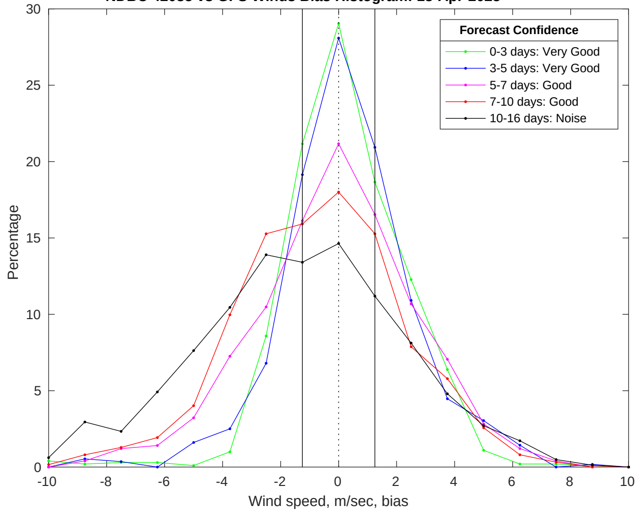
NDBC 42035 vs GFS Winds Bias Histogram: 13-Apr-2025
