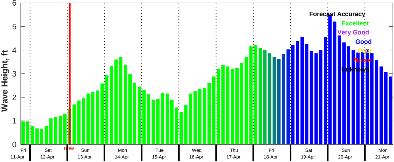
CMEMS Wave Forecast for NDBC 42035 from 11-Apr-2025 18:00:00 to 21-Apr-2025 18:00:00
