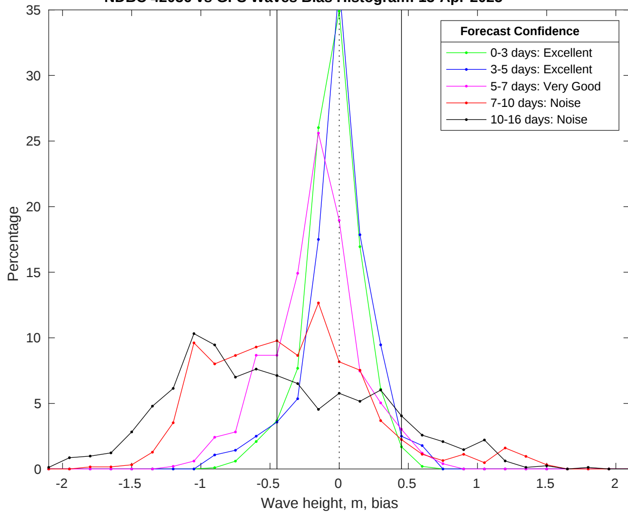
NDBC 42036 vs GFS Waves Bias Histogram: 13-Apr-2025
