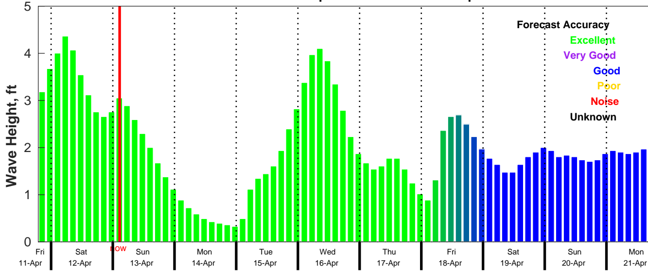
CMEMS Wave Forecast for NDBC 42036 from 11-Apr-2025 19:00:00 to 21-Apr-2025 19:00:00
