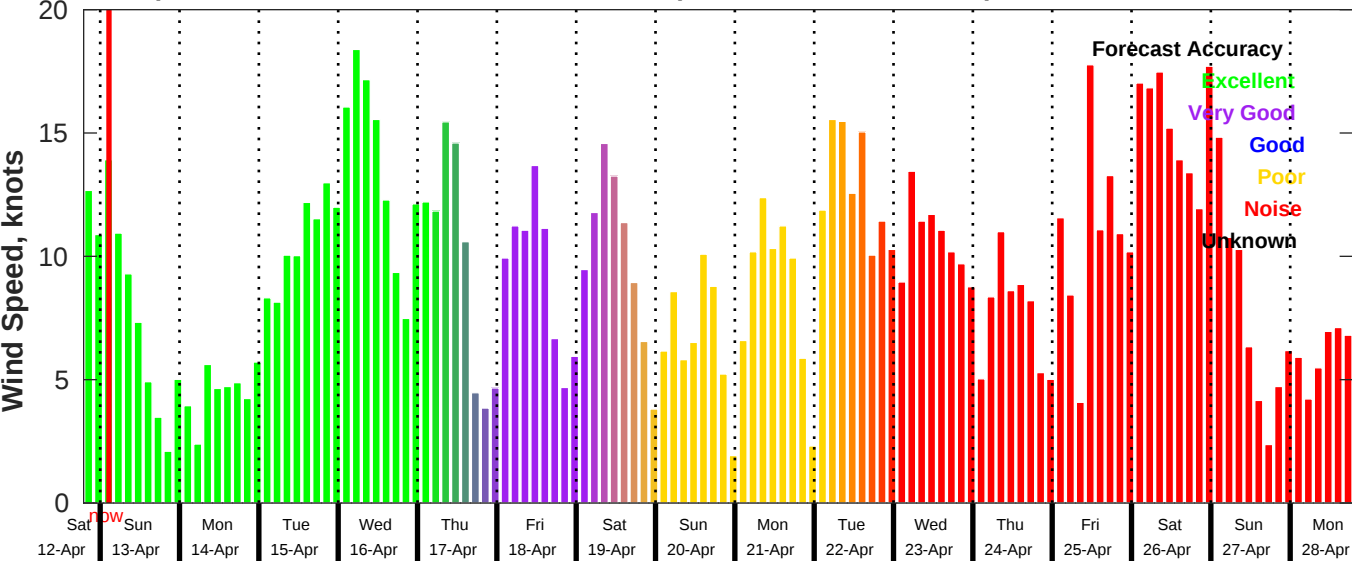
GFS Wind Speed Forecast for NDBC 42036 from 12-Apr-2025 19:00:00 to 28-Apr-2025 19:00:00
