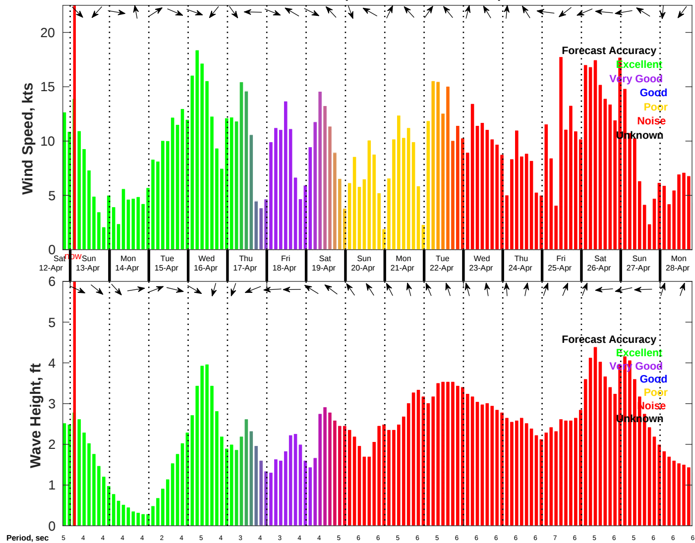
Wind & Wave Forecast for NDBC 42036 from 12-Apr-2025 19:00:00 to 28-Apr-2025 19:00:00
